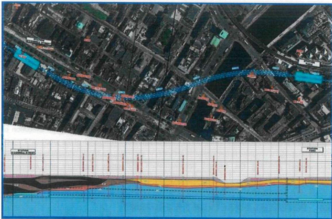
Figure 9. Geological Section
