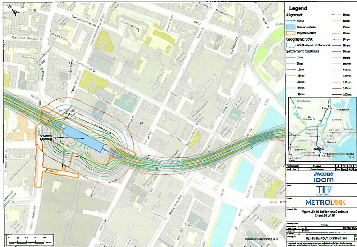
Figure 10. Settlement Contours (Extract from ML1-JAI-EIA-ROUT_XX-DR-Y-21146)
